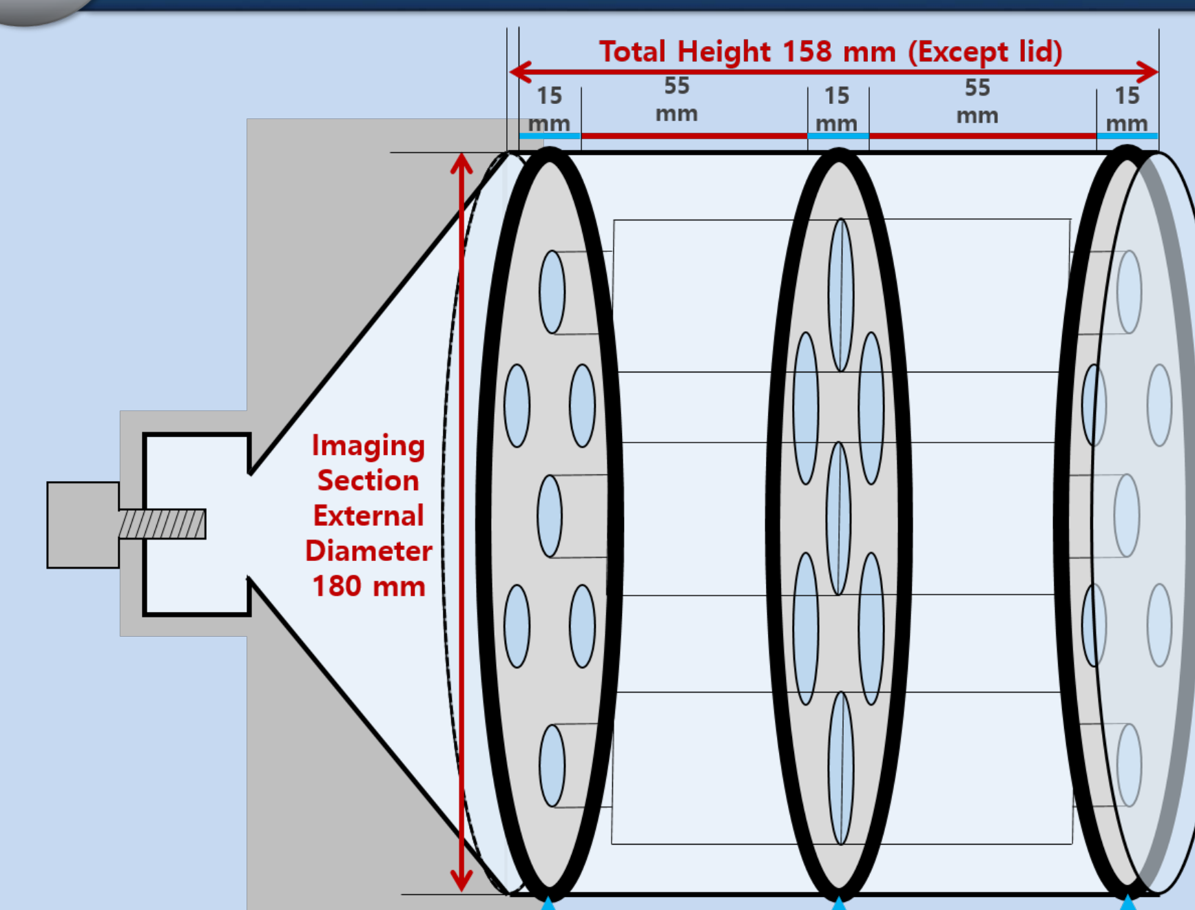
Fig.1 Geometry of the developed phantom: Total height and external diameter was decided by internal size of 8-channel MRI head coil. Two disks at both end and one disk in the middle of phantom can provide two different interspaces. 7 plugs can be located at one of the interspace between the disks. Thus, total 14 plugs can be inserted into phantom. The developed phantom was customized to fix 14 plugs without water leakage
